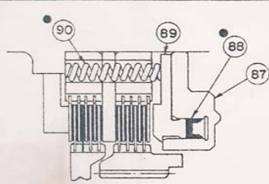
VIEW "A" ROTATED VIEW SHOWING FLYWHEEL BRAKE PISTON SPRING
